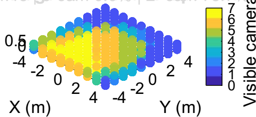
GA-best (Cost: 0.0179)
